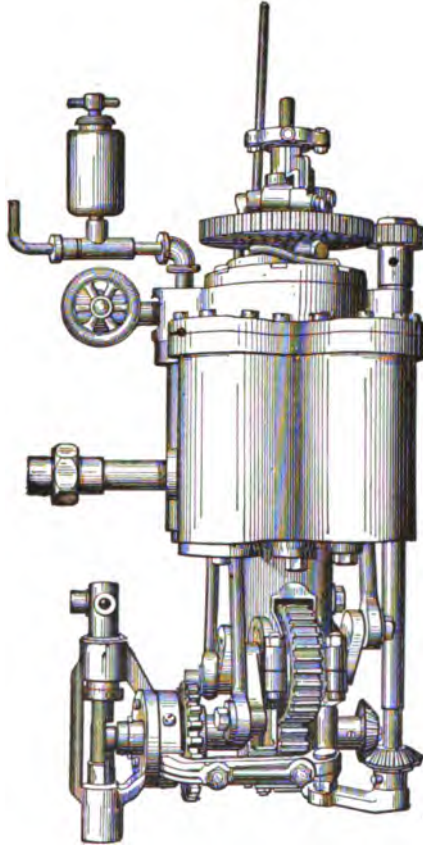
FIG. 202.—Engine of the "Reading" Steam Carriage.
